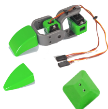
VR012: 2 servo leg
